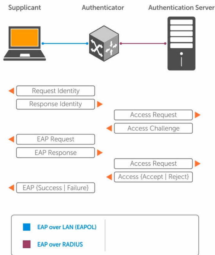
Figure 4. EAP Port-Authentication
